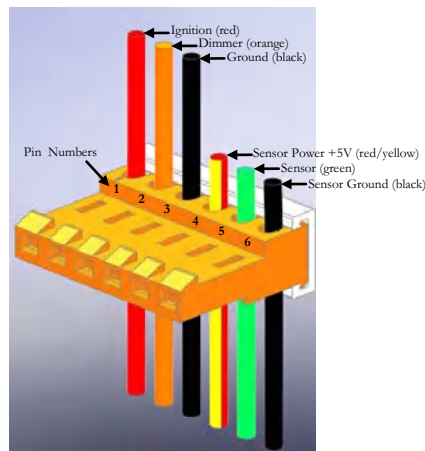
Figure 2: Connector.
