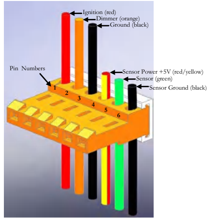
Figure 2: Connector.
